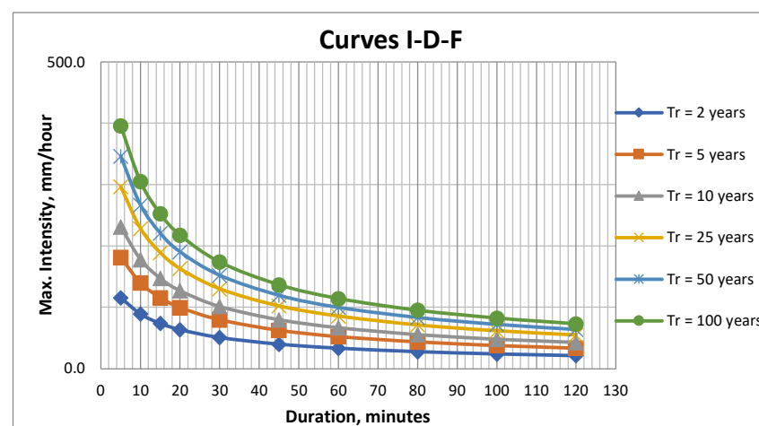
Figure 7. Intensity duration frequency curves.
