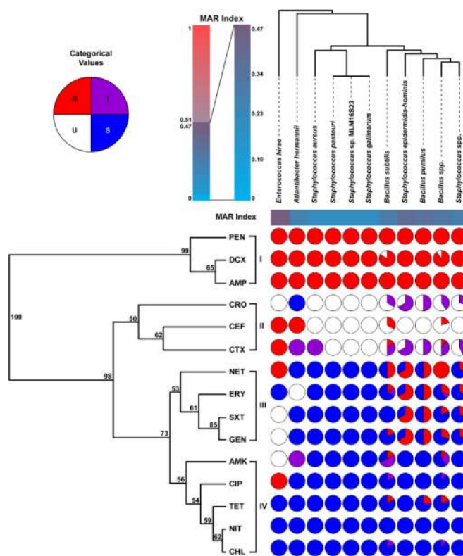
Figure 3. UPGMA-based hierarchical clustering and frequency heatmap of antibiotic susceptibility values for isolated bacteria.
