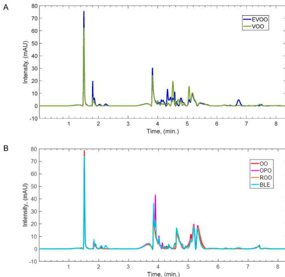
Fig. 1. Overlapped raw chromatograms of six olive oils considering one representative sample per olive oil category: A) EVOO and VOO, and B) OO, ROO, OPO and BLE. EVOO: extra virgin olive oil, VOO: virgin olive oil, OO: olive oil, ROO: refined olive oil, olive-pomace oil (OPO) and BLE: blend of EVOO or VOO with ROO or OPO.
